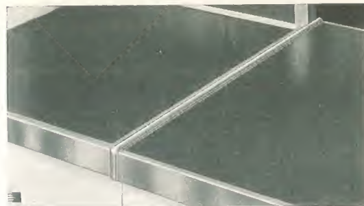
MS—MOULDING STRIP—Aluminum wedge seals crevice between linoleum sink top and adjacent base cabinet. Supplied with cement.
